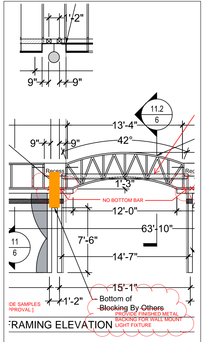
FIXTURE PLACEMENT @ AWNING
